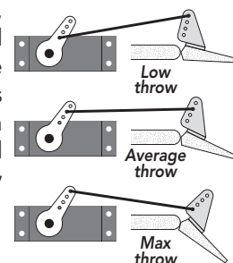
Aileron pushrod
